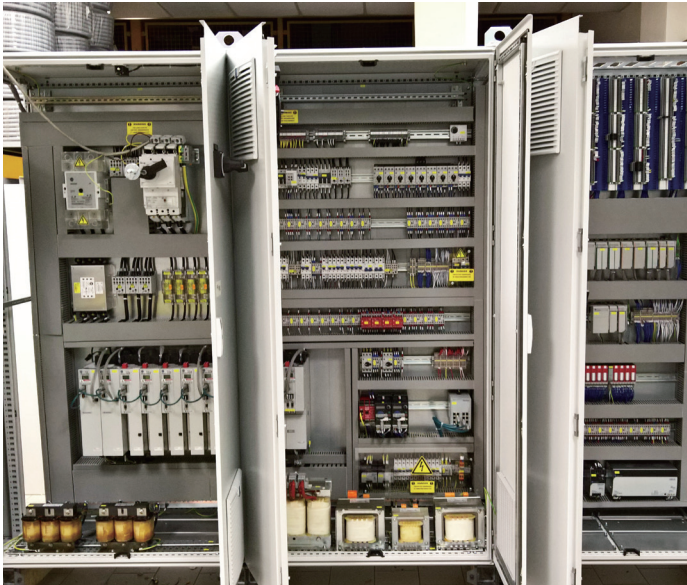
A control panel according to USA Standards
